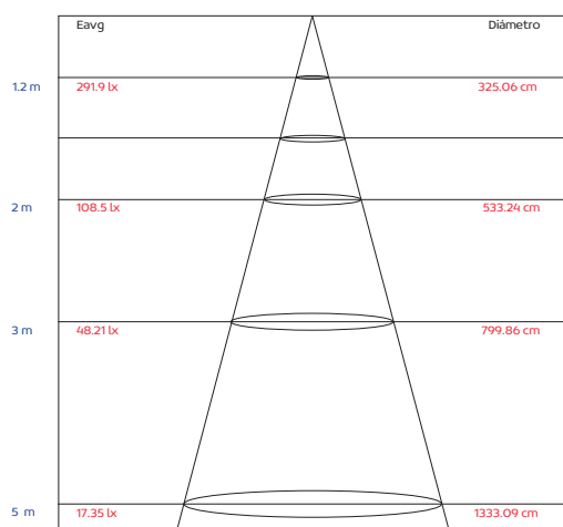
Lux-Distance Curve
